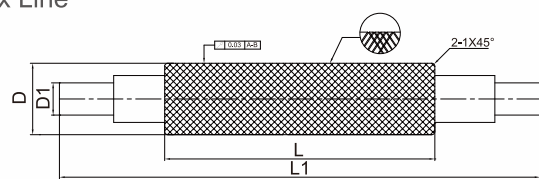
滚花 Anilox Line
