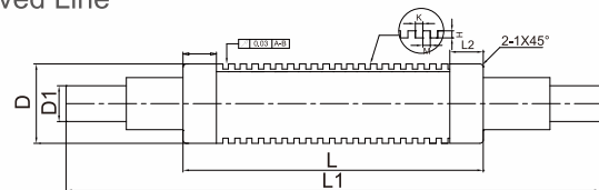
槽辊 Grooved Line
