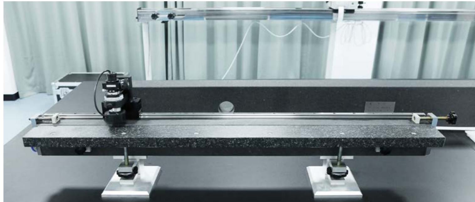
· 钢直尺检定装置 Steel Ruler Verification Device
